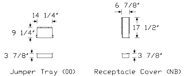
Jumper Tray (00)
